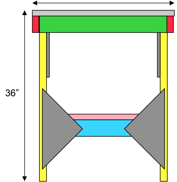
End View 2' 6"
